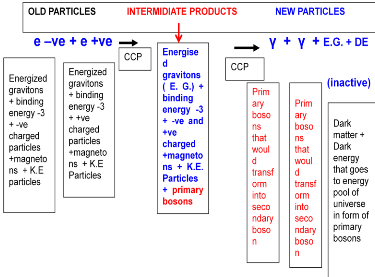
Fig 24 electron positron annihilation
