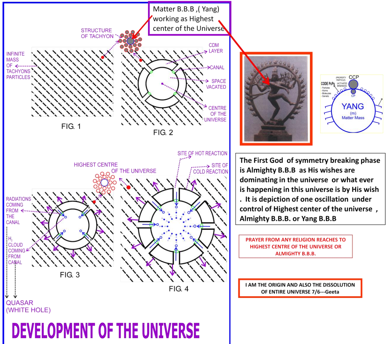
Figure 9.1 Hoyle Narlikar Universe
