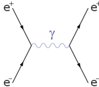
Fig 25 electron positron Annihilation -- wrong depiction
