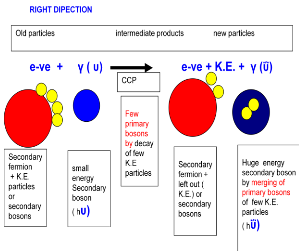
Fig 28 Inverse Compton scattering
