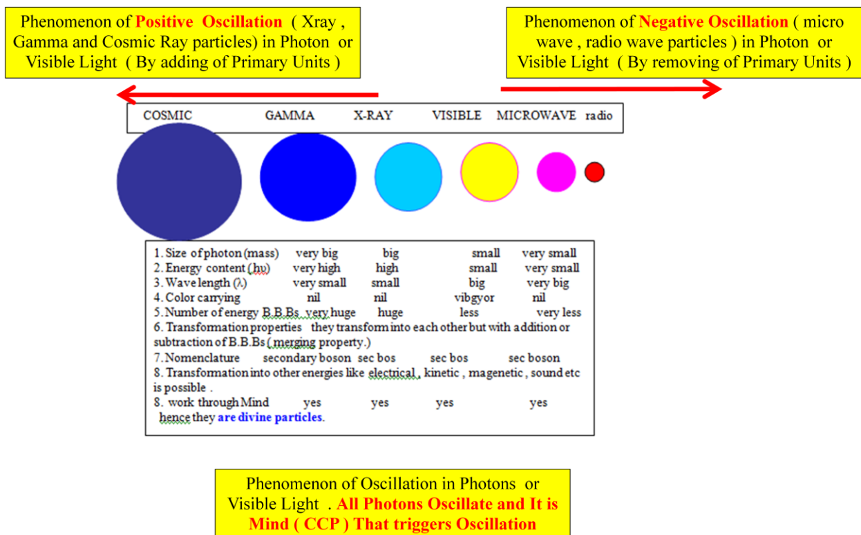
Fig 14 – Phenomenon of Oscillation in Photon
