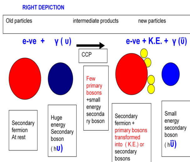
Fig- 29 Compton effect
