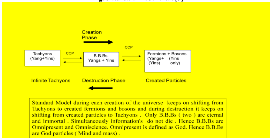
Fig. 3 standard Model chart [3]
