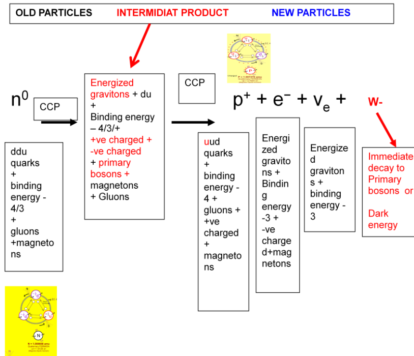
Fig 22 beta decay – Right Depiction
